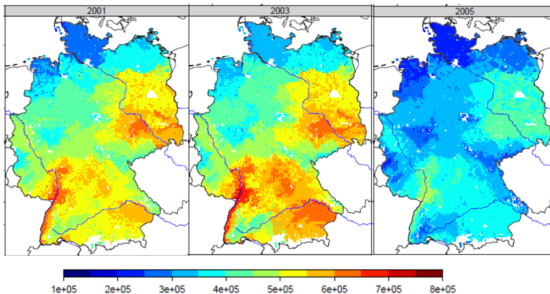
Fig. 3: Potential isoprene emission ( \mu\text{mol m}^{-2} \text{a}^{-1} ) inventory for three different years based on poplar short-rotation plantations fully covering the area of Germany.
