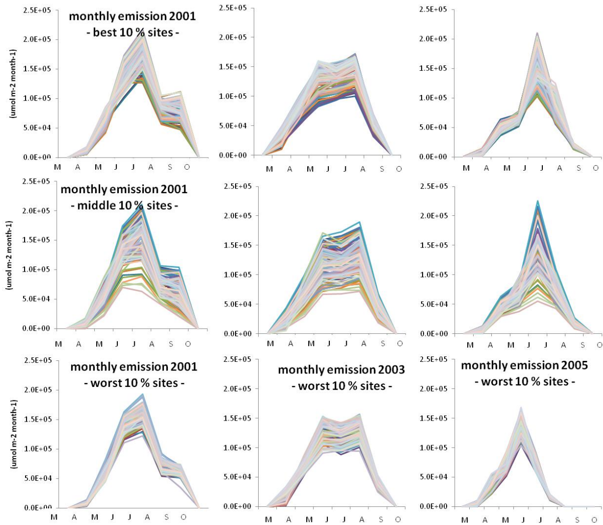
Fig. 2: Seasonal distribution of isoprene emission for 30 % of the investigated sites during three different years.
