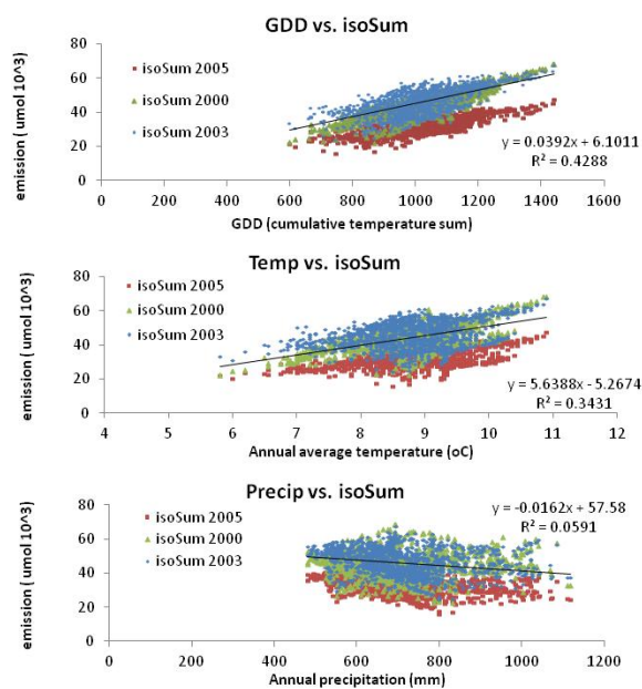
Fig. 1: Statistical relationships between environmental conditions and annual isoprene emission sums.
