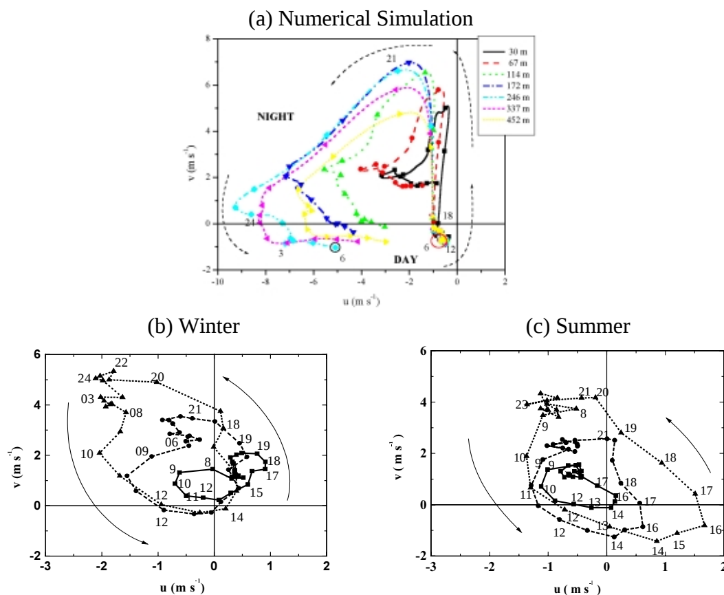
Figure 5 Wind hodograph (a) simulated numerically at 30, 67, 114, 172, 246, 337 and 452 m; (b) observed during winter (c) summer at 10, 60 and 80m (squares, circles and triangles) in Iperó. The numbers indicate local time.
