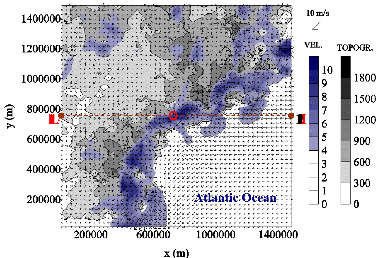
Figure 2 Horizontal wind field at 15 m above the surface at 03:00 LT. The wind velocity at 337 m above the surface is indicated by blue scale. Topography is indicated by gray scale. The red open circle in the center indicates position of Iperó. Letters A and B define the position of the cross section displayed in Figure 3.
