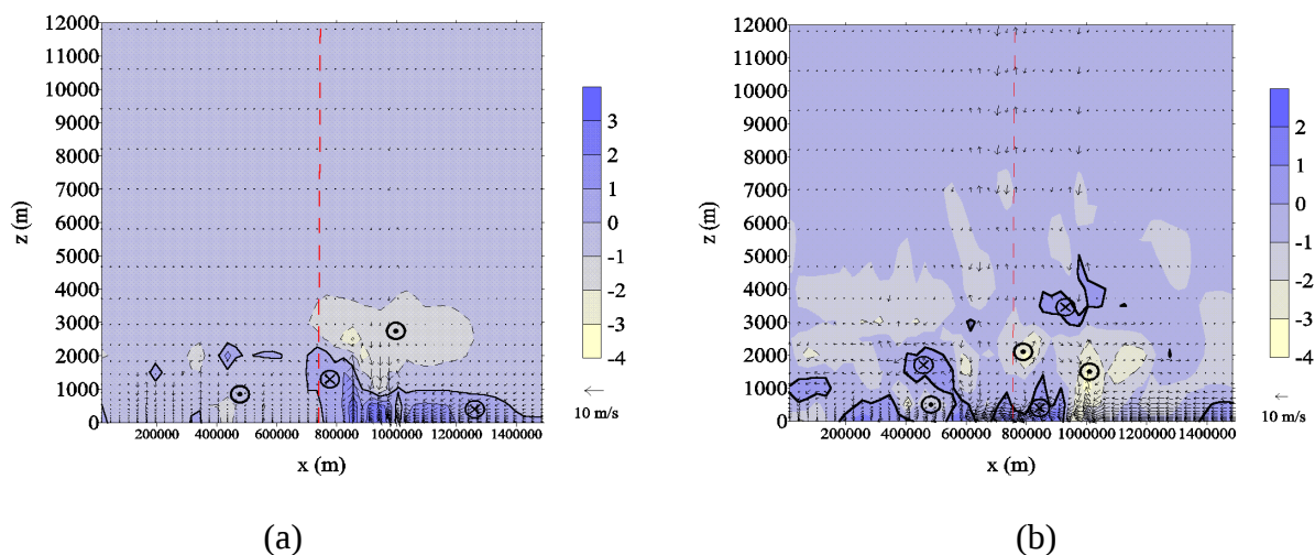
Figure 3 Meridional component of the wind vector (blue-yellow scale) simulated at (a) 18:00 LT and (b) 03:00 LT, along the line AB in Figure 1 and 2). The wind vector ( u , 100 \cdot w ) is present also. The vertical dashed red line indicates Iperó.
