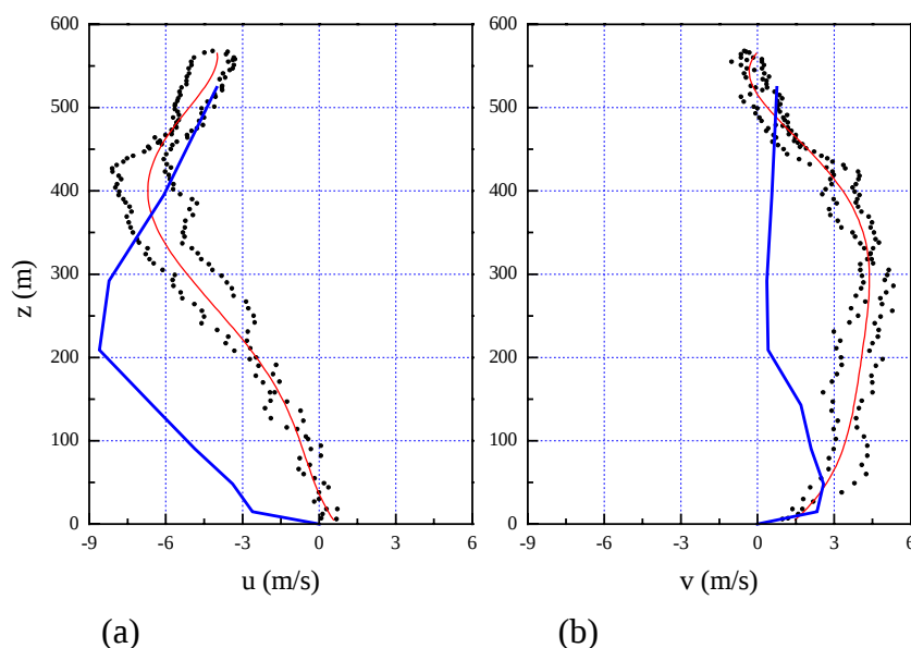
Figure 4 (a) Zonal and (b) meridional wind speed components associated with a nocturnal low-level jet observed during winter at Iperó, Brazil at 03:00 LT. The bold lines indicate the simulation.
