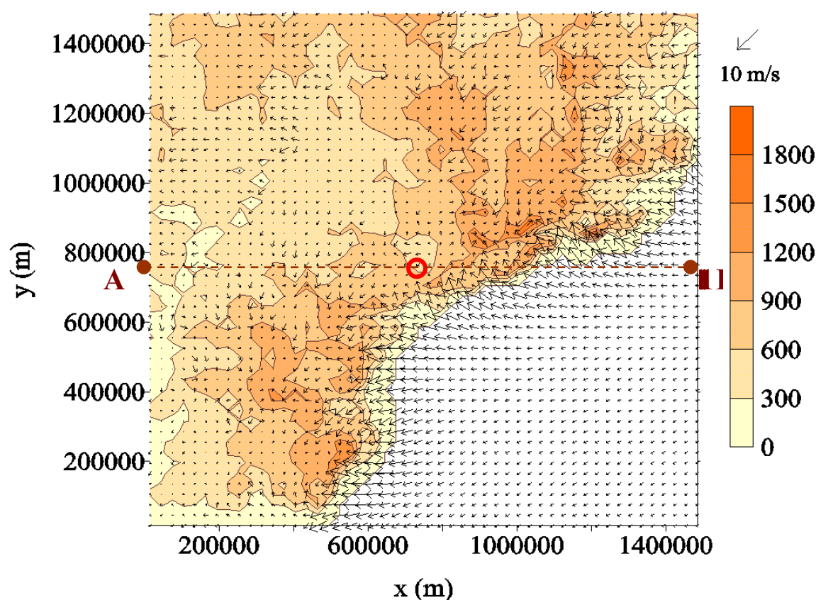
Figure 1 Horizontal wind field at 15 m above the surface at 18:00 LT. Topography is indicated by orange scale. The red open circle in the center indicates position of Iperó. Letters A and B define the position of the cross section displayed in Figure 3.
