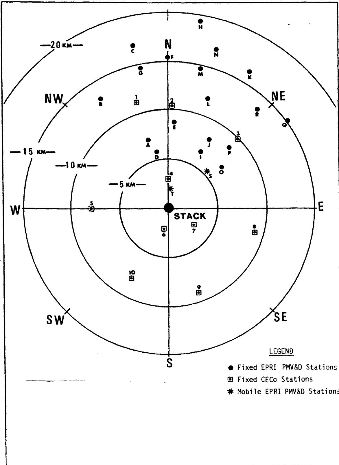
Figure 4-2. EPRI PMV&D and CECo air quality monitoring network - Plains Site field experiment.
